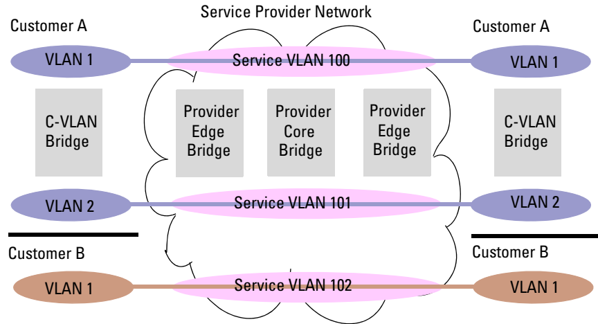
Figure 8-2. Example of VLANs in a QinQ Configuration
