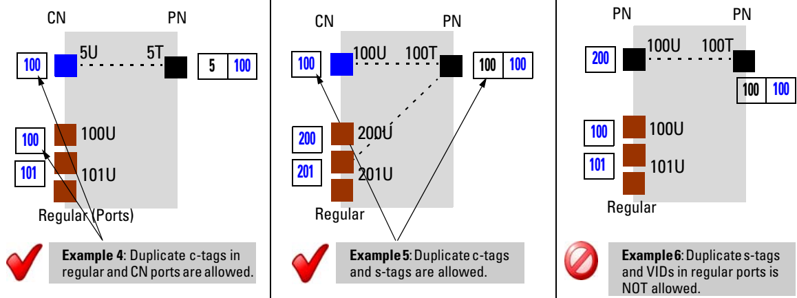
Figure 8-4. QinQ and Duplicate VID's: Examples of Allowed Configurations
