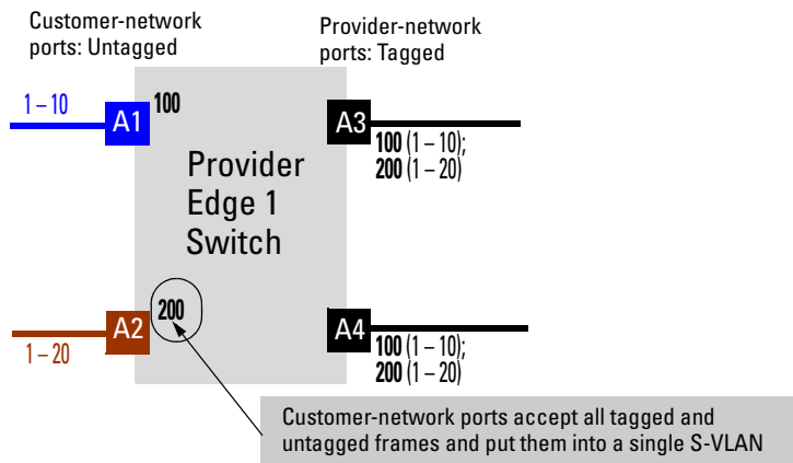
Figure 8-7. Configuration Example: Edge Switch 1
